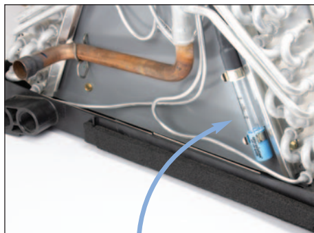
Lamp and cable assembly with magnet-mounts allows many options for lamp positioning
